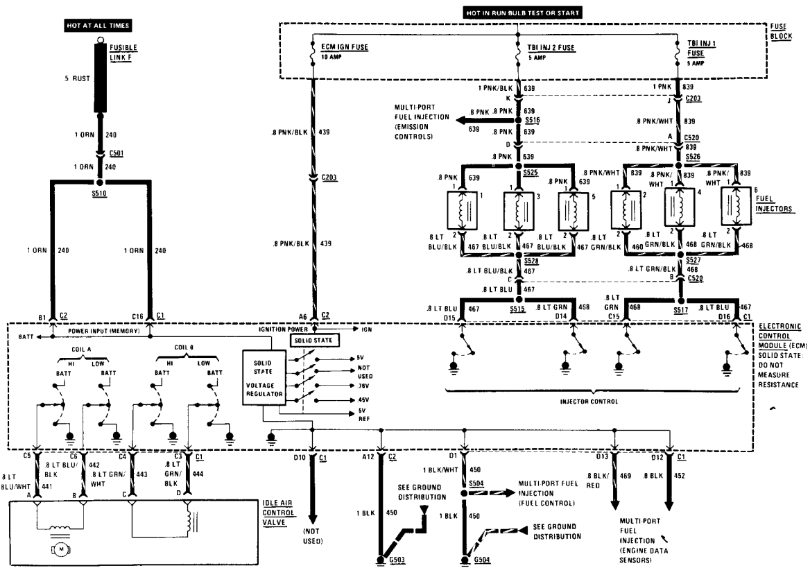
Multi-port fuel injection (V6 engine) — fuel injectors
