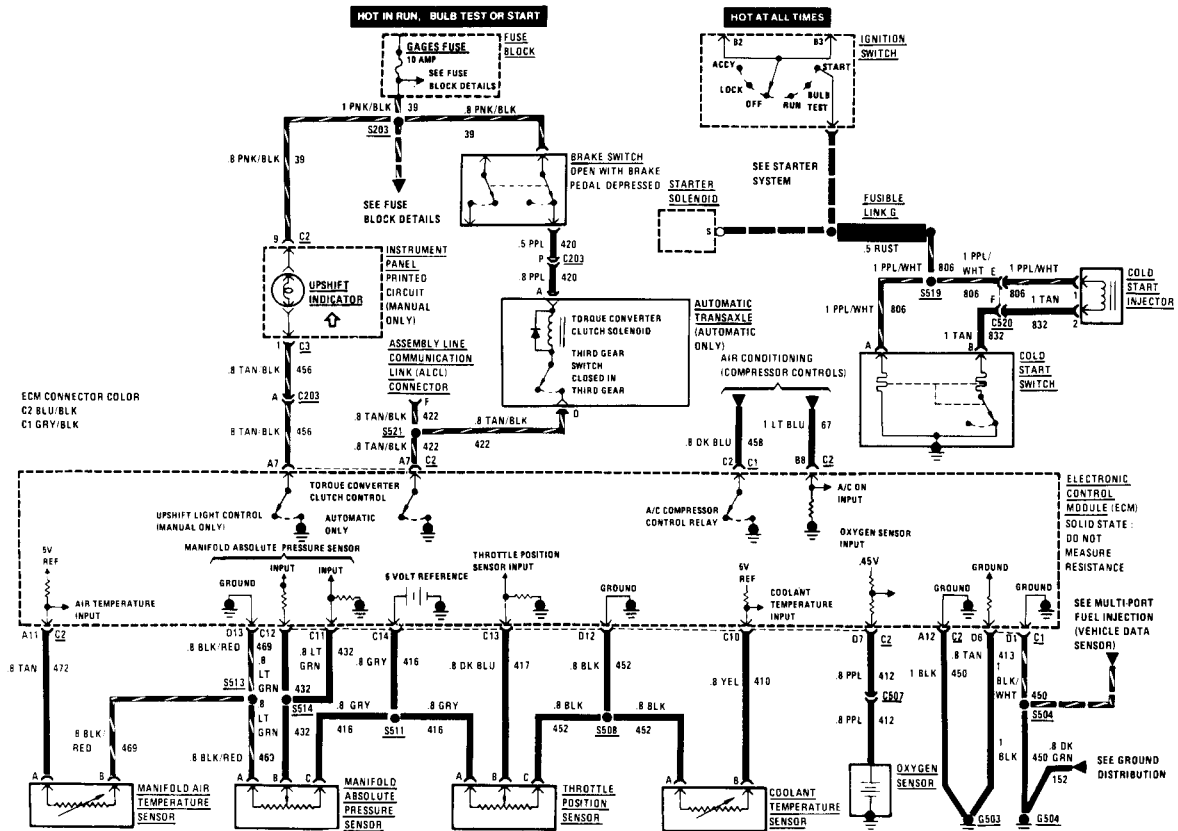
Multi-port fuel injection (V6 engine) — engine data sensors, Torque Converter Clutch (TCC) and cold start injector
