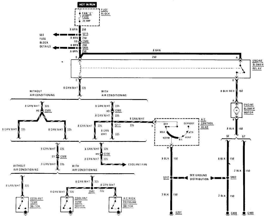
Coolant fan – engine blower assembly (V6 engine)
