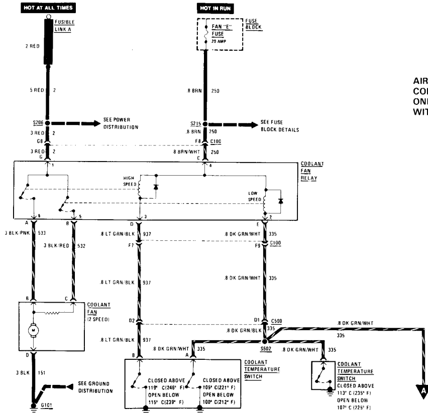
Coolant fan – two-speed (four-cylinder engine)
