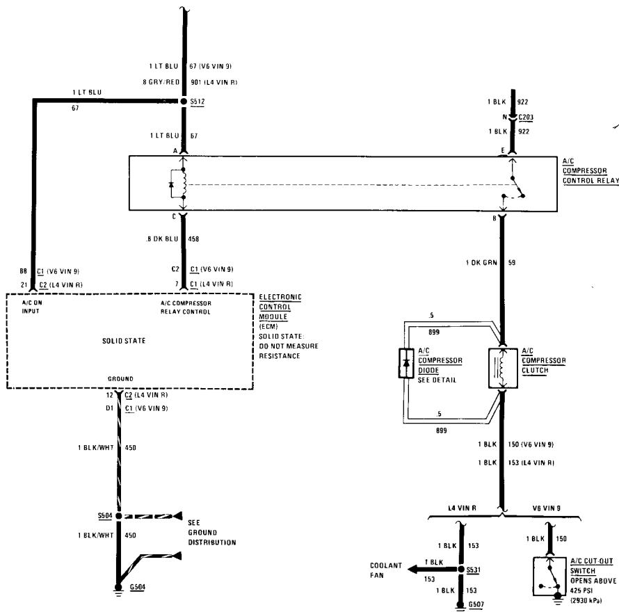
Air conditioning system — compressor controls
